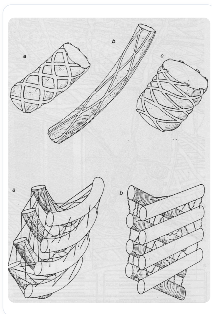
FIG. — Tensegrity
